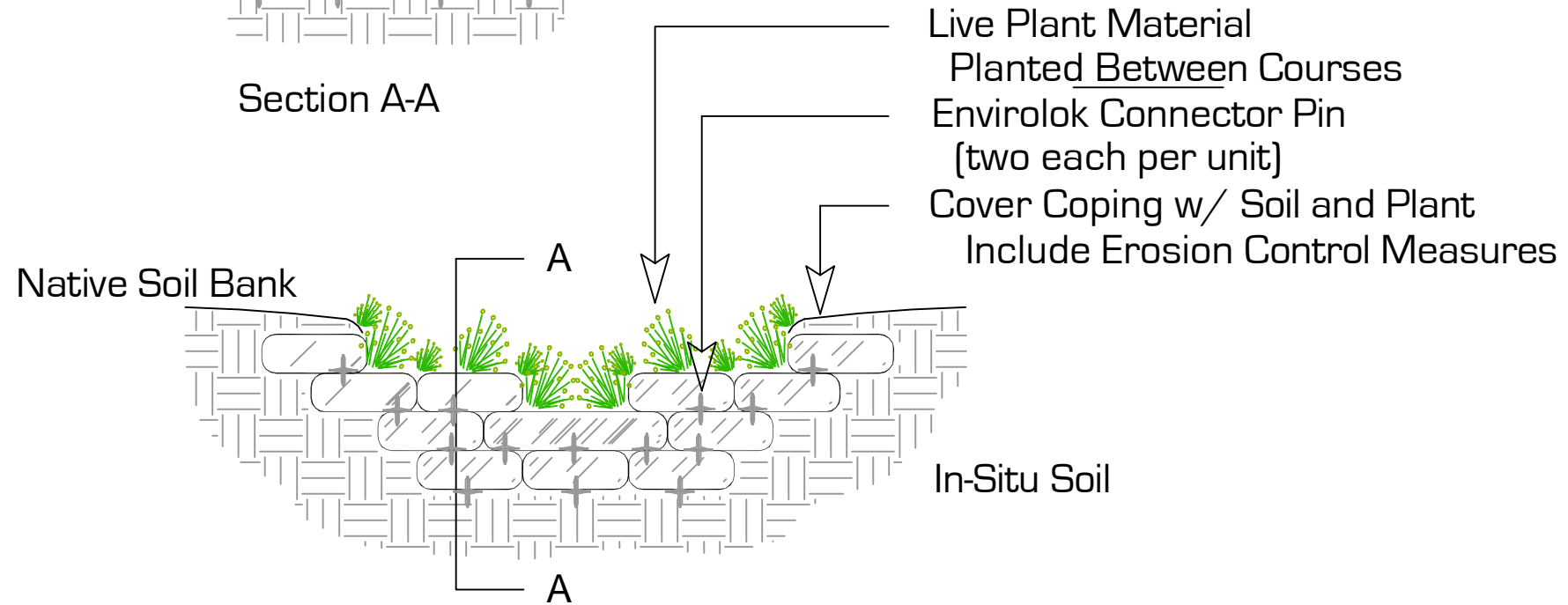
CROSS SECTION
