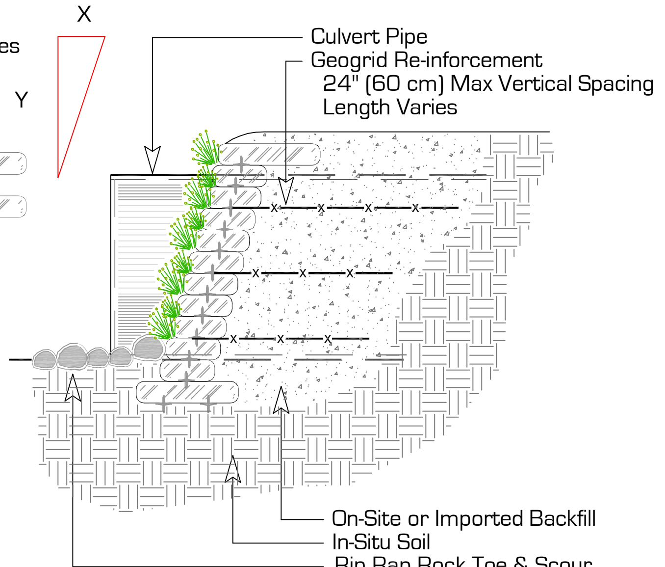
SECTION
