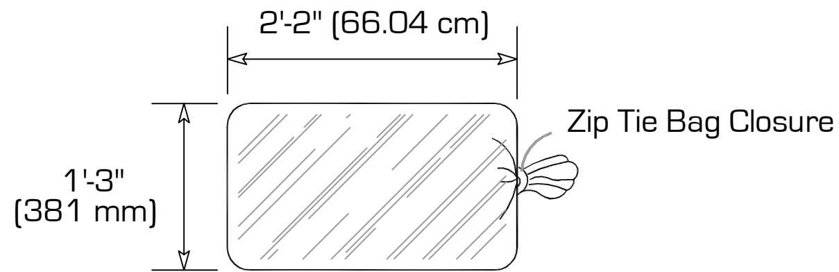
PLAN VIEW
